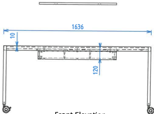
Front Elevation
