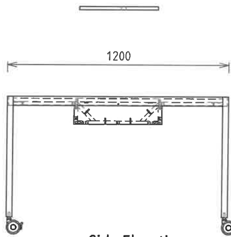
Side Elevation
